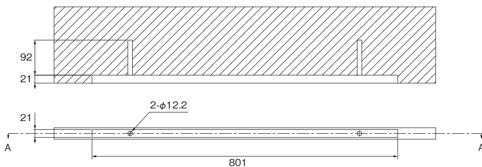
Reference diagram for shelf digging dimensions
