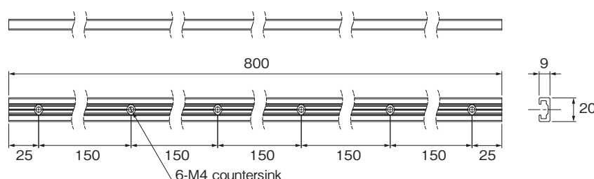
K217-800-SL-A L800 (with holes)
